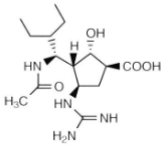
Peramivir
